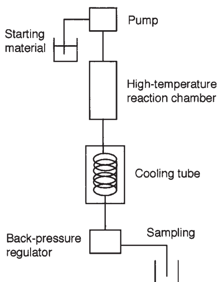
Fig. 1. Scheme of the flow reactor system.
